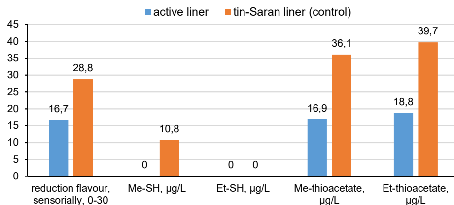
Figure 5: Development of the contents of VSCs and of sensorially perceptible reduction flavour after 8 months of bottle storage (upright, dark, 20° C) after sealing with screwcaps fitted with different liners.
