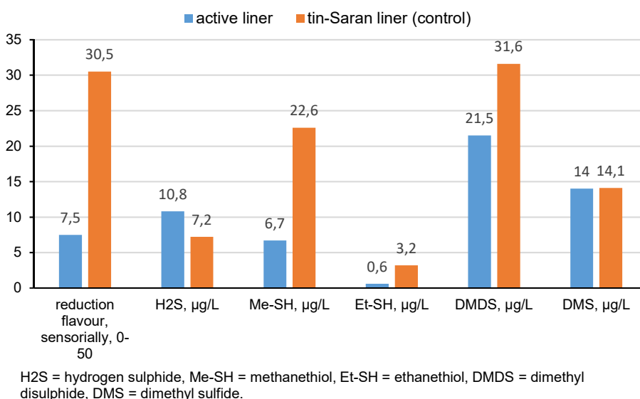
Figure 4: Development of the contents of VSCs and of sensorially perceptible reduction flavour of a tainted wine (Chardonnay) after 8 months of bottle storage (upright, dark, 20° C) after sealing with screwcaps fitted with different liners.
