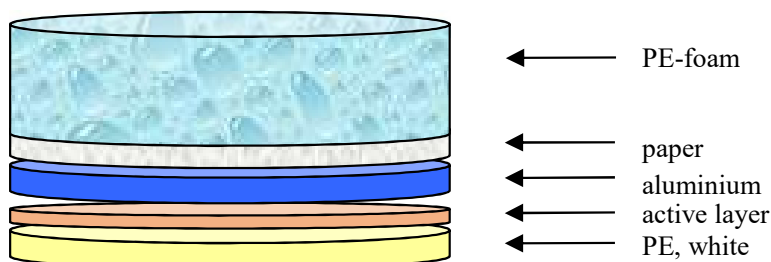
Figure 3: Structure of a VSCs-absorbing liner for screwcaps.
